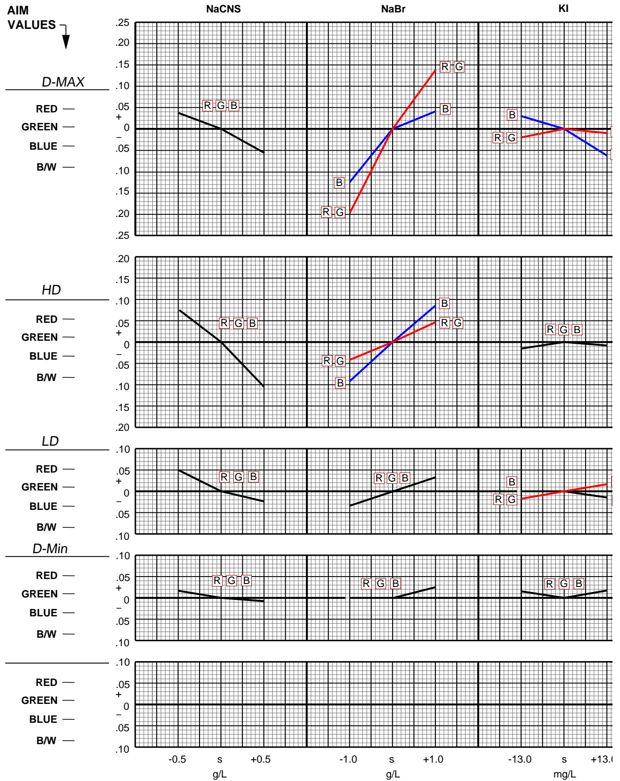
Figure 12-10 Effects of NaCNS, NaBr and KI Variations—7399 Film in Process VNF-1 First Developer
