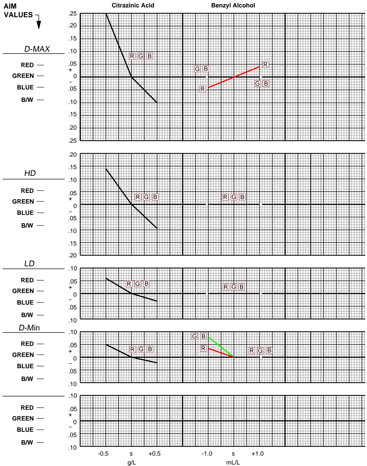
Figure 12-7 Effects of Citrazinic Acid and Benzyl Alcohol Variations—7240 Film in Process VNF-1 Color Developer
