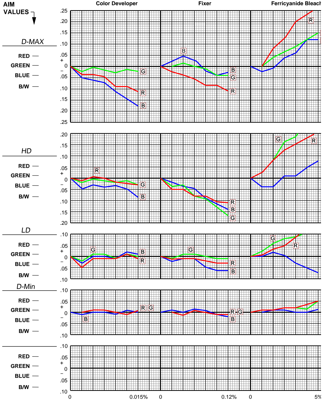
Figure 12-15 Effects of Color Developer, Fixer and Ferricyanide Bleach Contamination —7240 Film in Process VNF-1 First Developer
