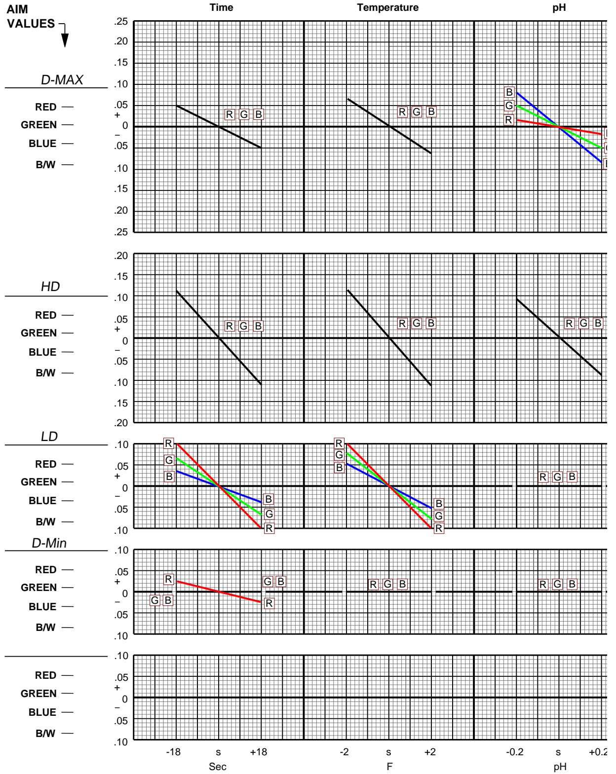
Figure 12-2 Effects of Time, Temperature and pH Variations—7240 Film in Process VNF-1 First Developer
