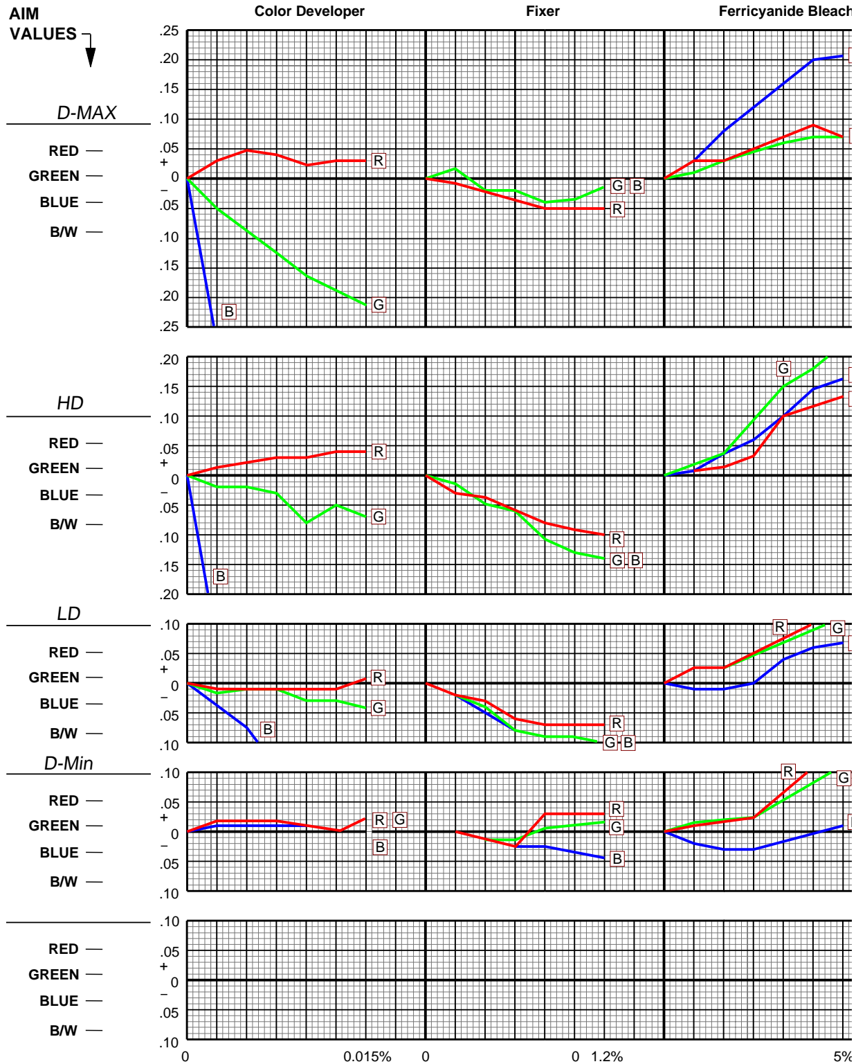
Figure 12-19 Effects of Color Developer, Fixer and Ferricyanide Bleach Contamination —7399 Film in Process VNF-1 First Developer
