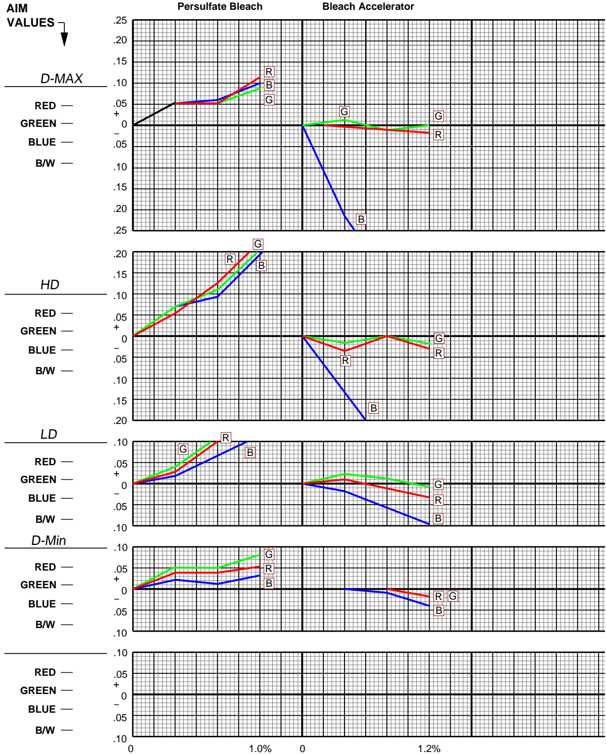
Figure 12-16 Effects of Persulfate Bleach and Bleach Accelerator Contamination —7240 Film in Process VNF-1 First Developer
