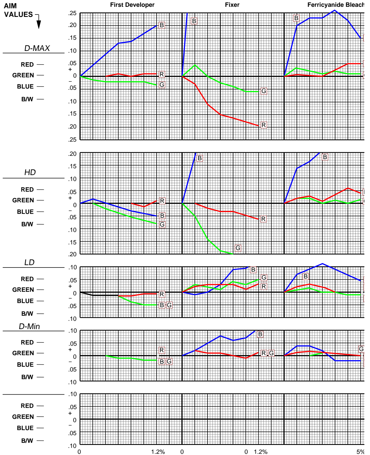
Figure 12-21 Effects of First Developer, Fixer and Ferricyanide Bleach Contamination —7399 Film in Process VNF-1 Color Developer
