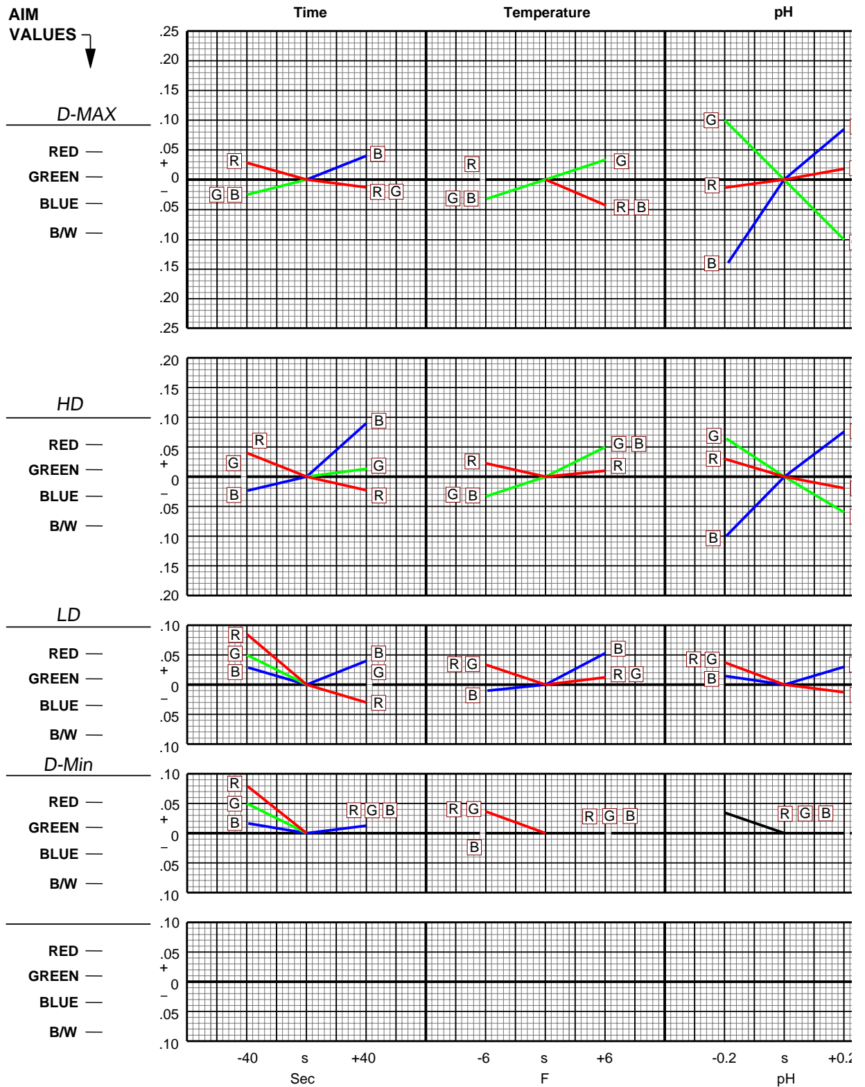
Figure 12-11 Effects of Time, Temperature and pH Variations—7399 Film in Process VNF-1 Color Developer
