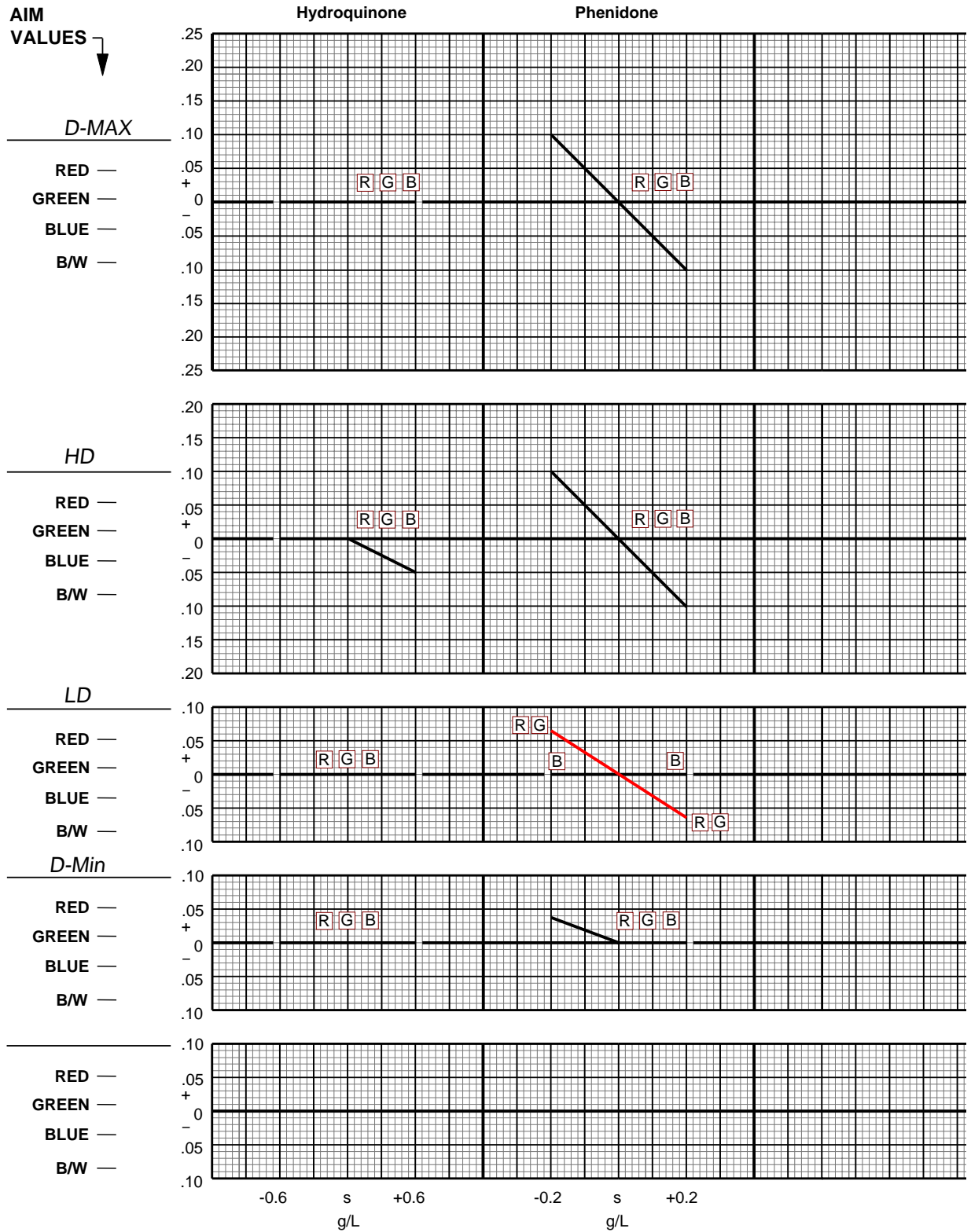
Figure 12-3 Effects of Hydroquinone and Phenidone Variations—7240 Film in Process VNF-1 First Developer
