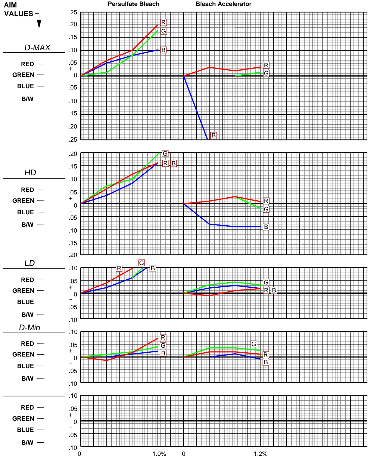
Figure 12-20 Effects of Persulfate Bleach and Bleach Accelerator Contamination —7399 Film in Process VNF-1 First Developer
