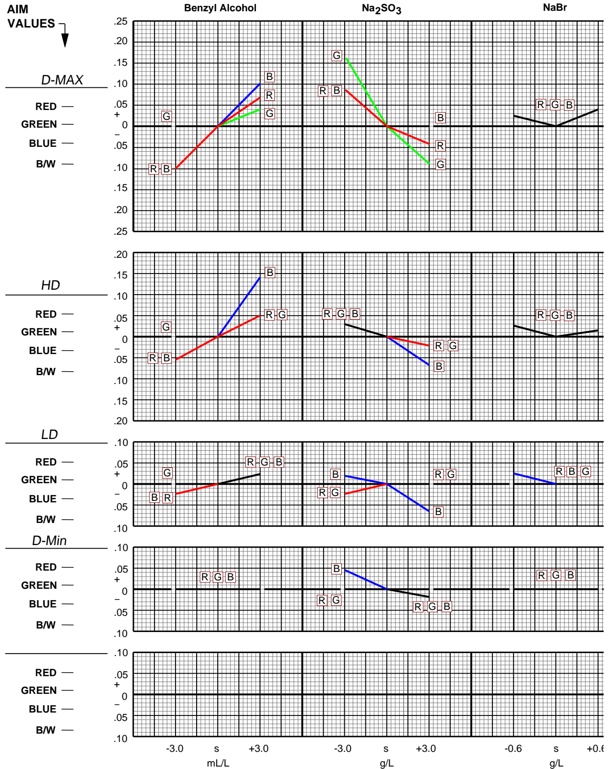
Figure 12-12 Effects of Benzyl Alcohol, Na 2 SO 3 and NaBr Variations—7399 Film in Process VNF-1 Color Developer
