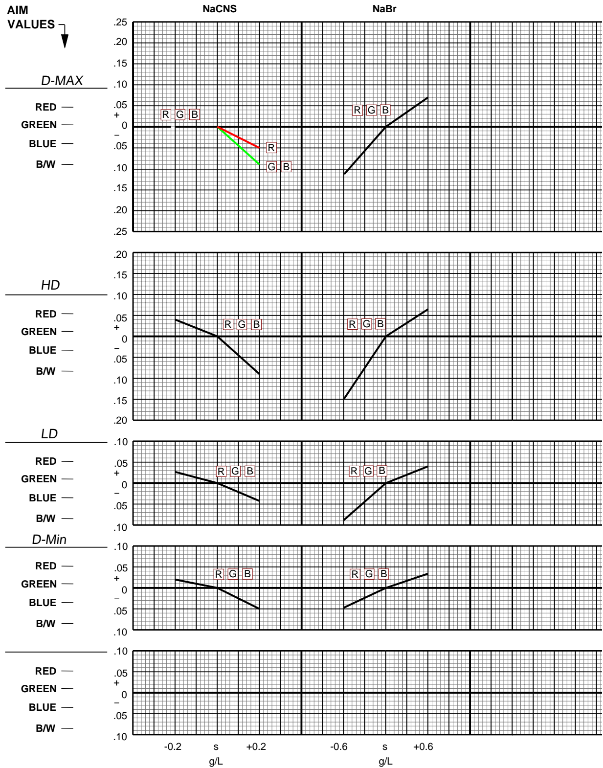
Figure 12-4 Effects of NaCNS and NaBr Variations—7240 Film in Process VNF-1 First Developer
