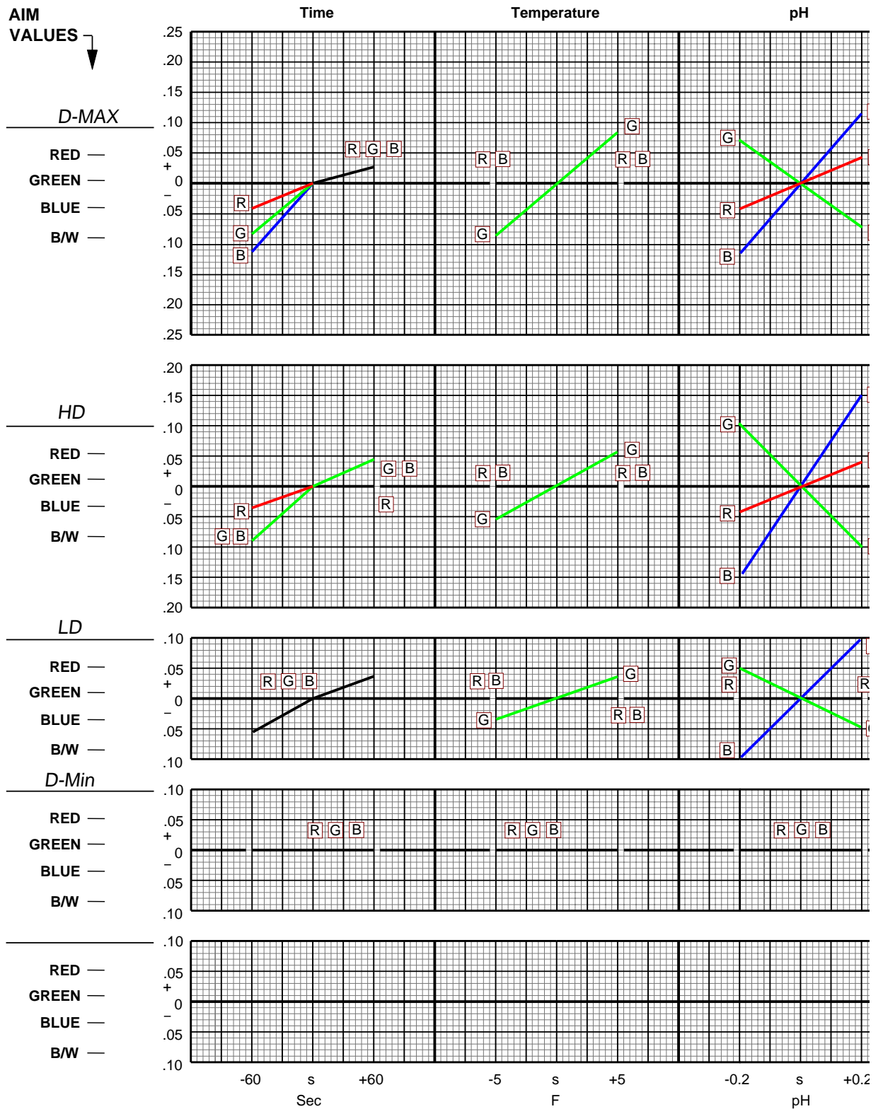
Figure 12-5 Effects of Time, Temperature and pH Variations—7240 Film in Process VNF-1 Color Developer
