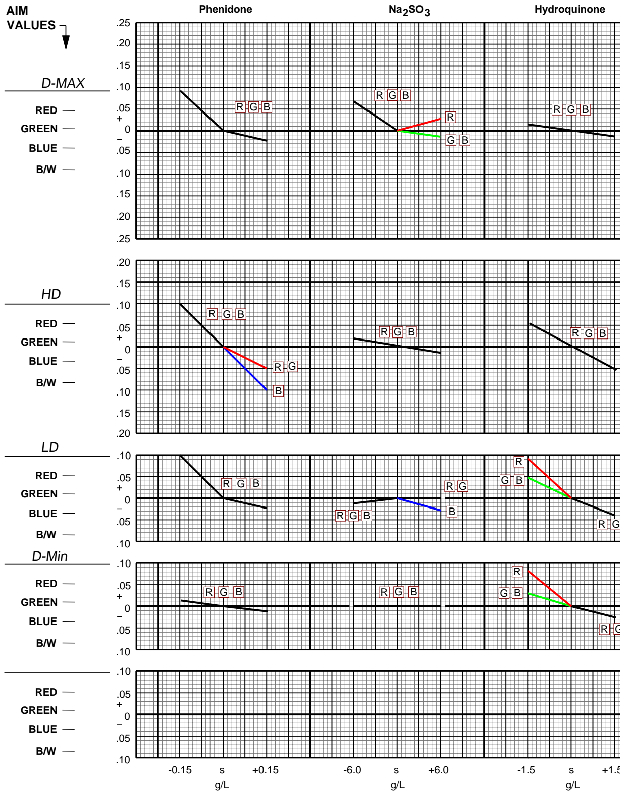
Figure 12-9 Effects of Phenidone, Na 2 SO 3 and Hydroquinone Variations—7399 Film in Process VNF-1 First Developer
