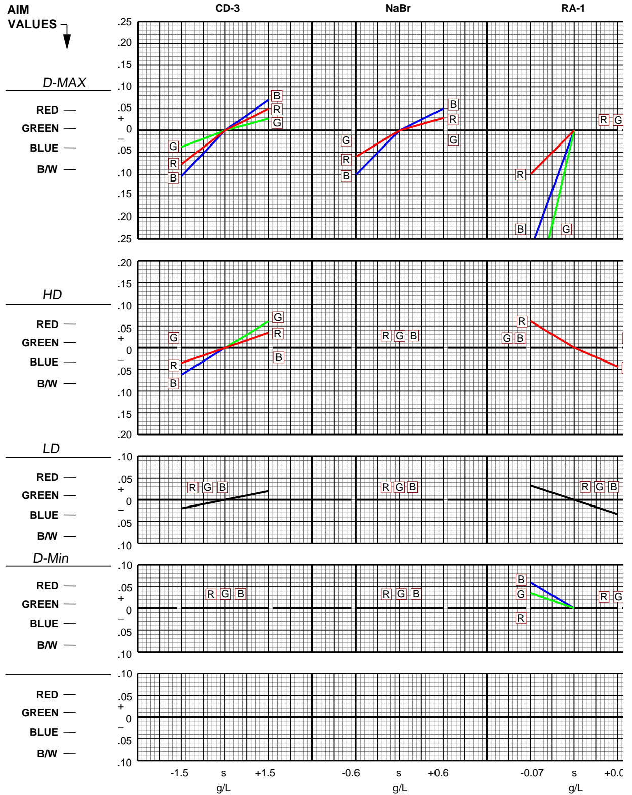
Figure 12-6 Effects of CD-3, NaBr and RA-1 Variations—7240 Film in Process VNF-1 Color Developer
