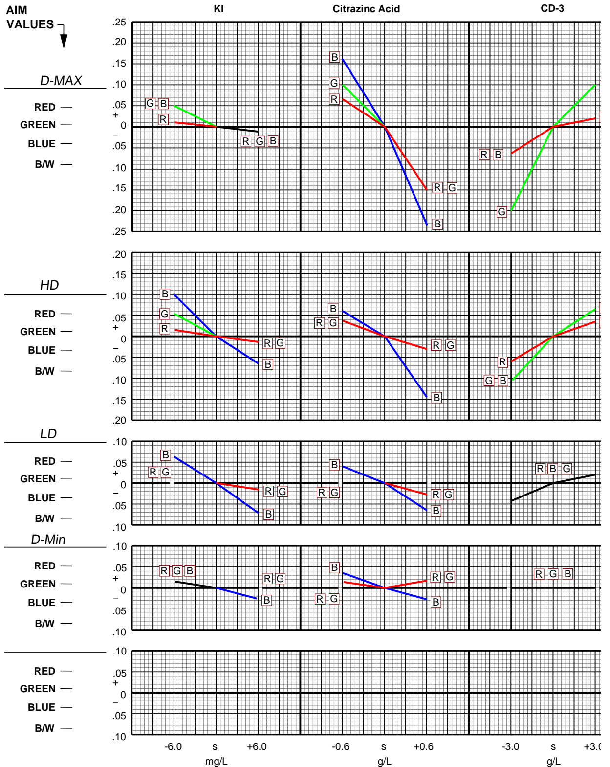
Figure 12-13 Effects of KI, Citrazinc Acid and CD-3 Variations—7399 Film in Process VNF-1 Color Developer
