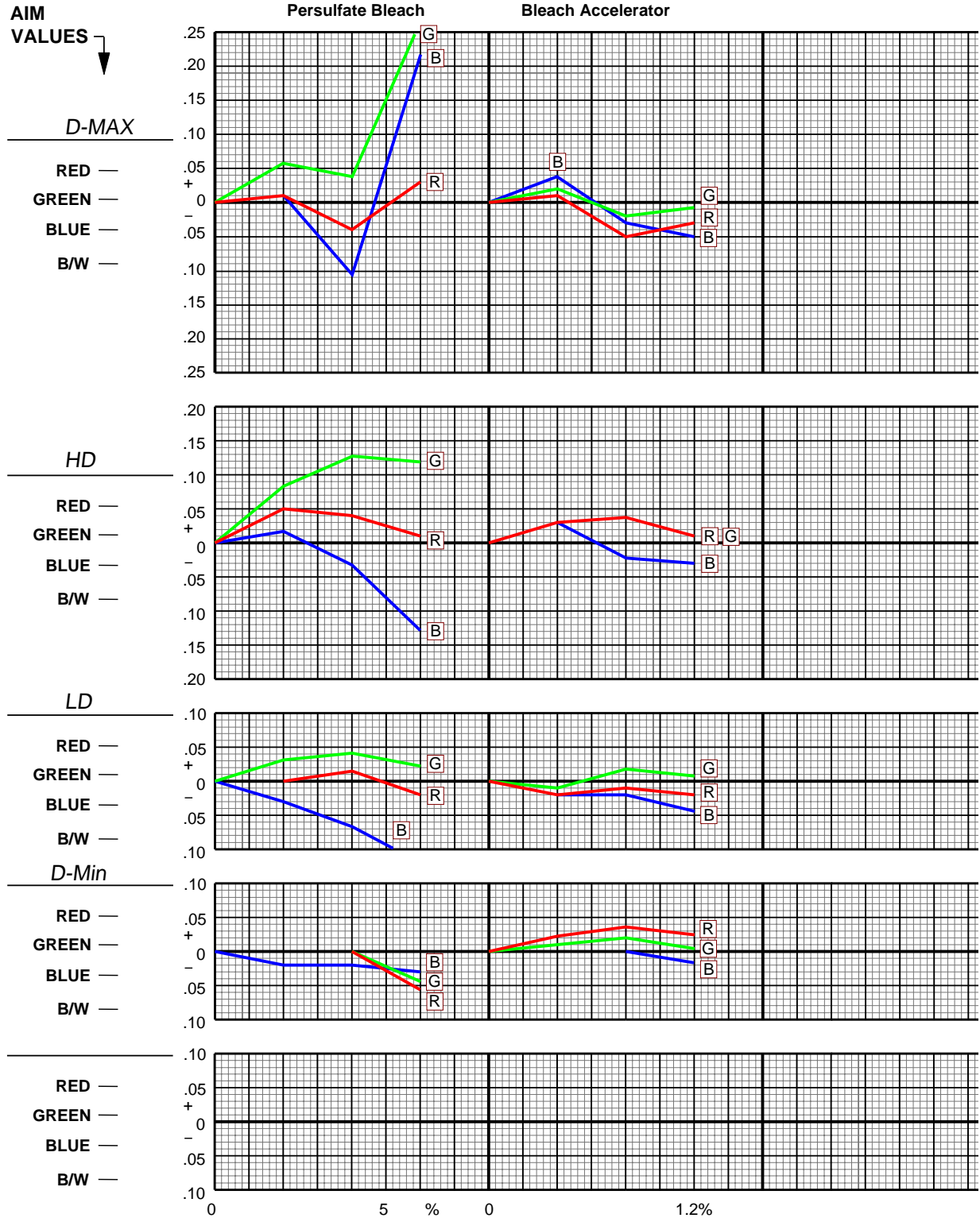
Figure 12-18 Effects of Persulfate Bleach and Bleach Accelerator Contamination —7240 Film in Process VNF-1 Color Developer
