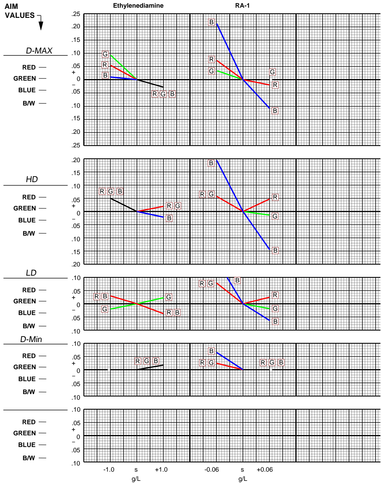
Figure 12-14 Effects of Ethylenediamine and RA-1 Variations—7399 Film in Process VNF-1 Color Developer
