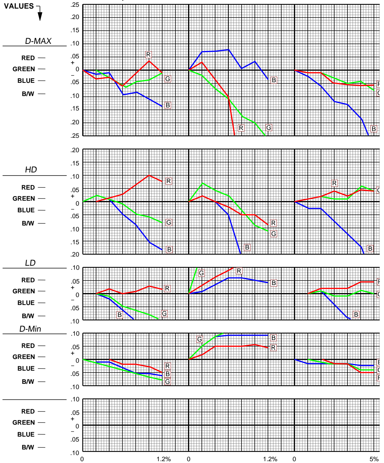
Figure 12-17 Effects of First Developer, Fixer and Ferricyanide Bleach Contamination —7240 Film in Process VNF-1 Color Developer
