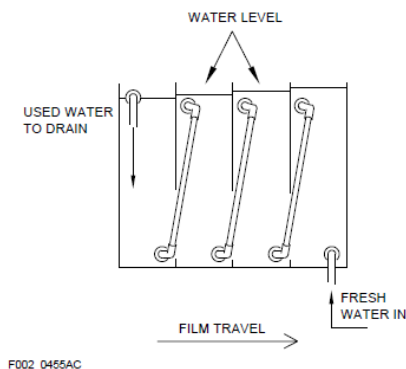
Figure 7-3 Four-Stage Countercurrent Wash
