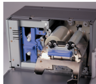
RIMAGE writers not only automatically load, record and stack discs but even print the label
