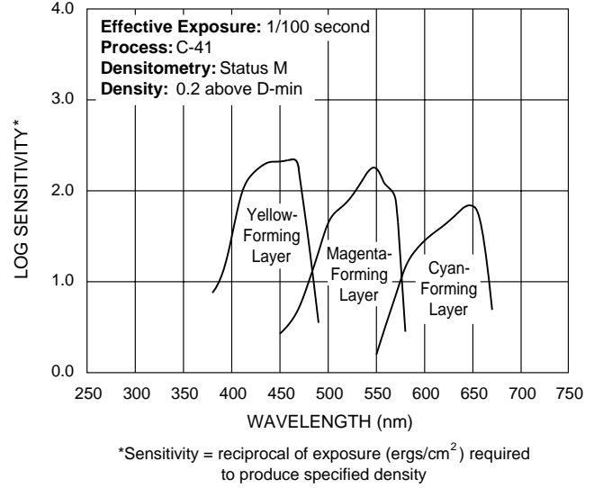
Spectral-Sensitivity Curves
