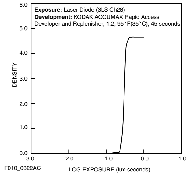
Characteristic Curve
