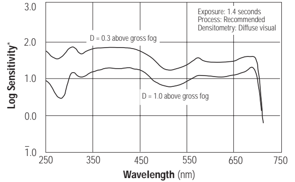
Spectral Sensitivity
