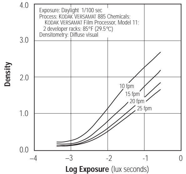
Characteristic Curves
