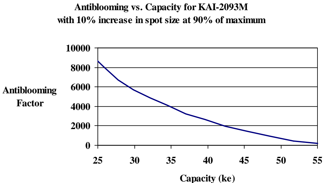
Figure 2: Antiblooming Vs. Capacity
