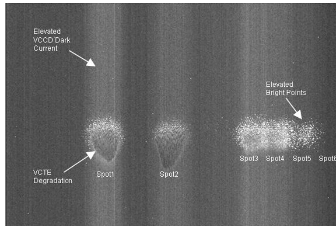
Figure 3: Examples of Damage to a KAI-16000 Device due to Bright Spot Exposures
